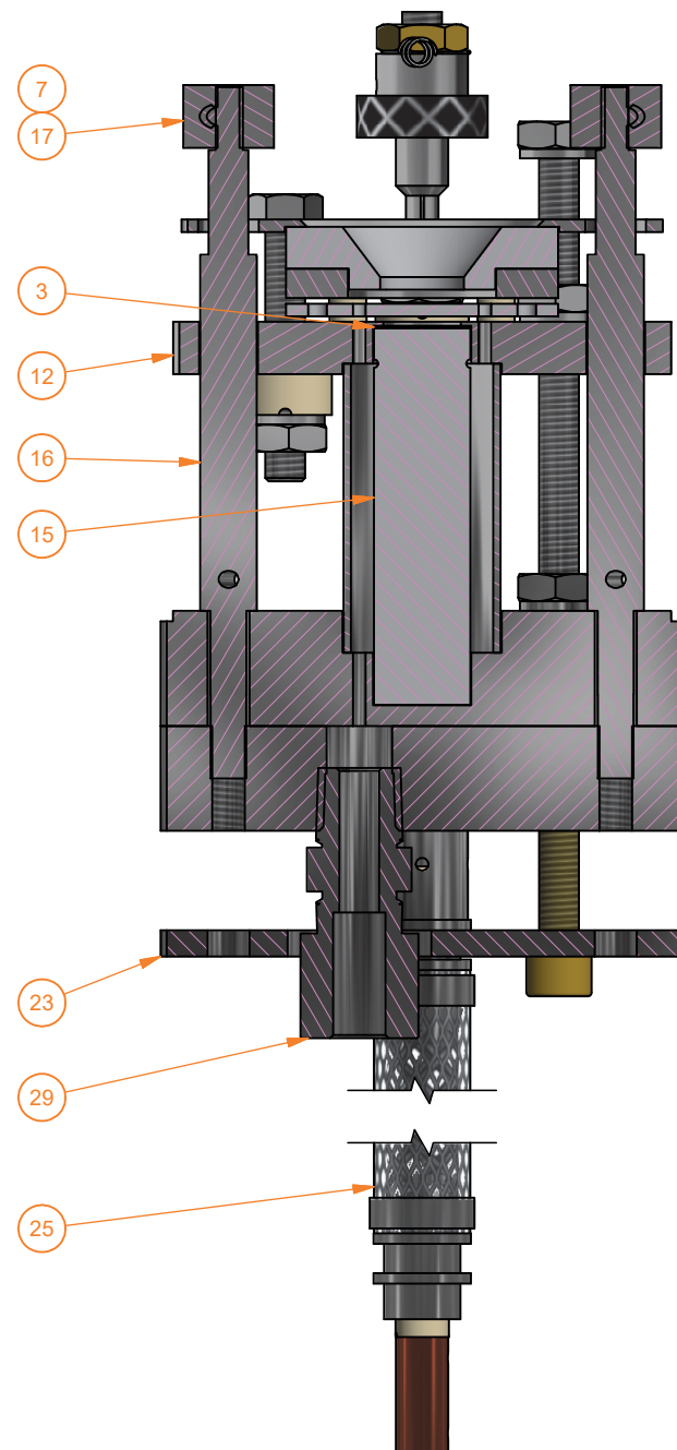
SECTION B-B SCALE 1 / 1
