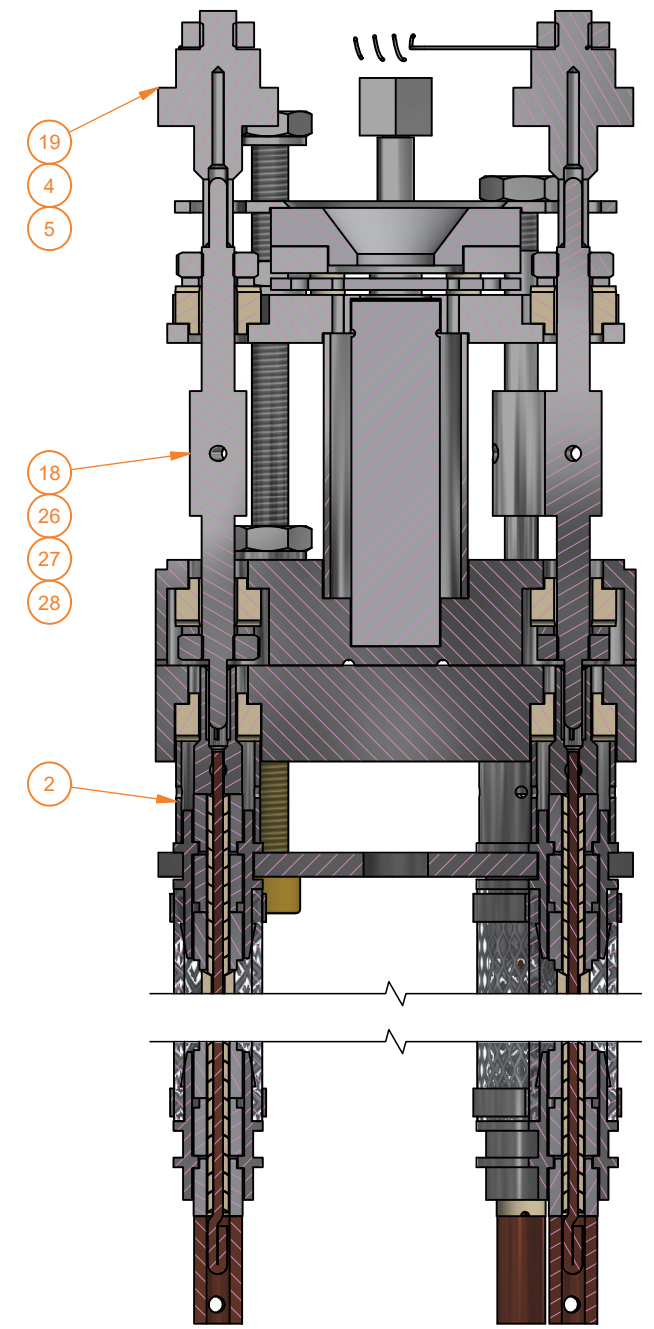
SECTION D-D SCALE 1 / 1
