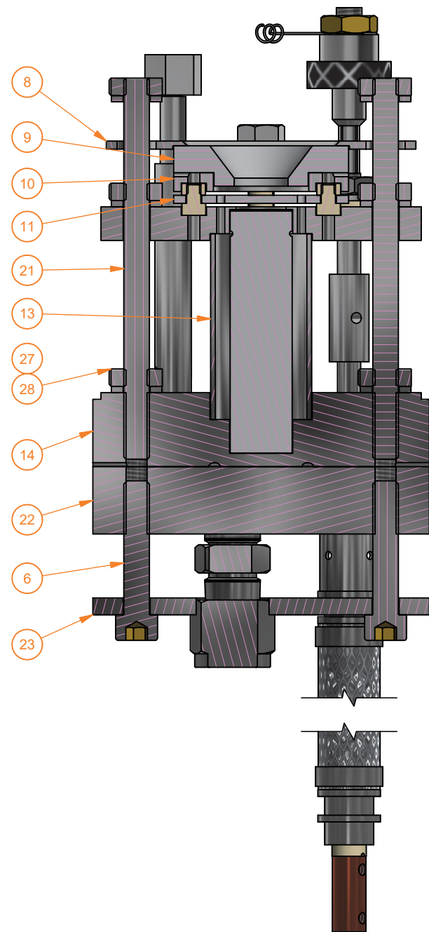
SECTION A-A SCALE 1 / 1
