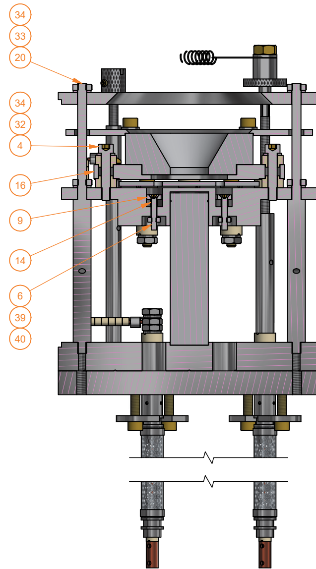
SECTION C-C SCALE 1:2
