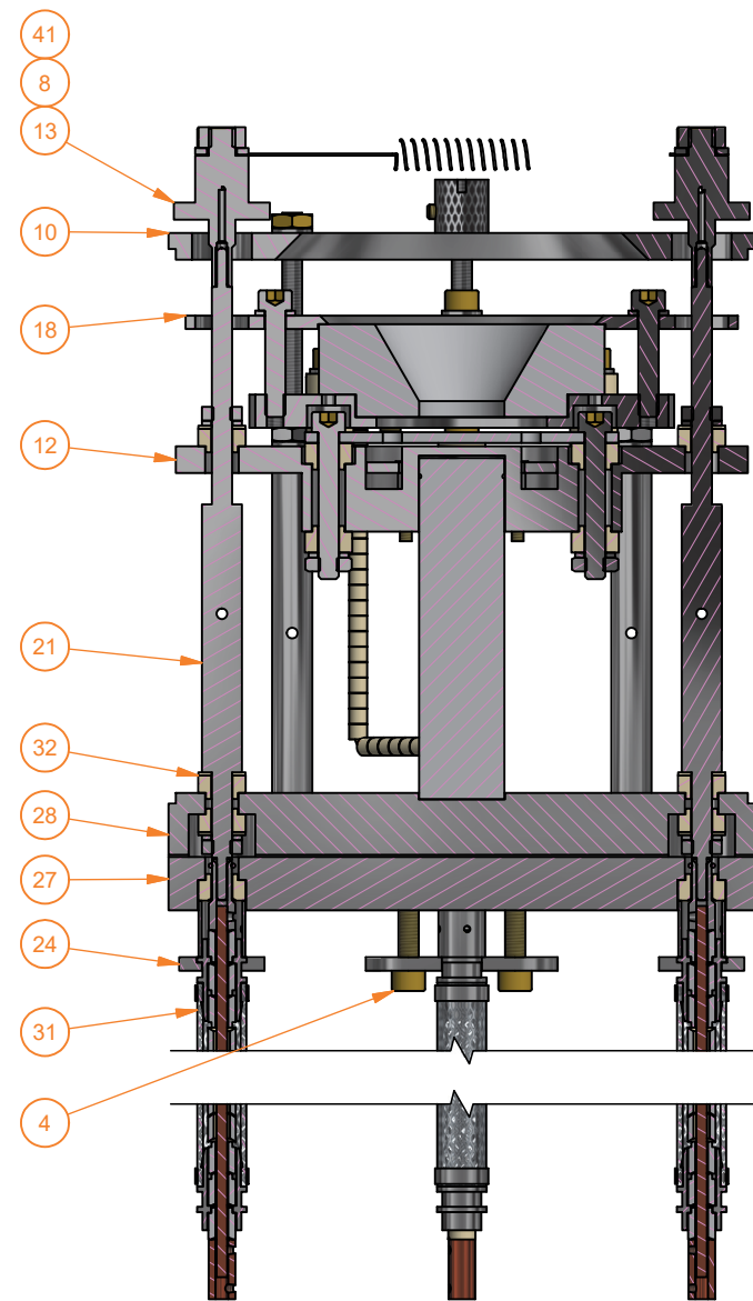
SECTION B-B SCALE 1:2
